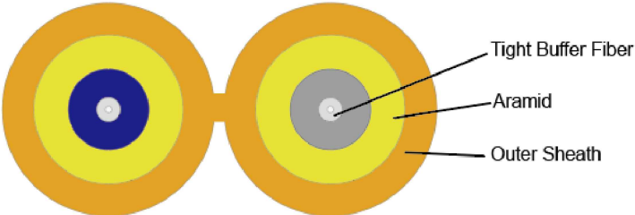
Cable Structure
