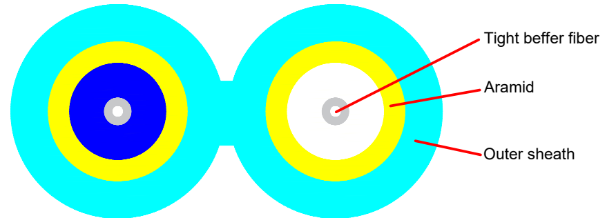
Cable Structure
